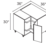
CORNER WITH LAZY SUSAN 36" | BC36LS(L/R)
