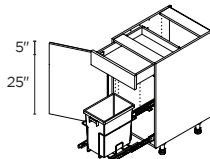
PULL-OUT / 1 DOOR / 1 DRAWER 18" | B18PWB(L/R)
