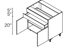
2 DOORS / 1 DRAWER / 1 FIXED FRONT 36" | BCT36BFF
