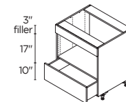
1 DRAWER 30" | BMW30
