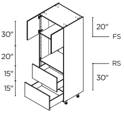
MICROWAVE 1 2 DOORS / 2 DRAWERS 30" | TO2D3084.5
