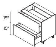
2 DRAWERS / 1 INNER DRAWER 36" | BCT2D36II
