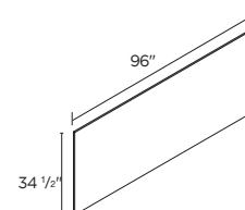
ISLAND PANEL 34 1/2"
