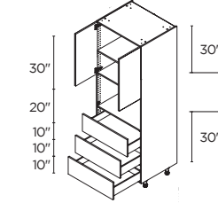
MICROWAVE 1 2 DOORS / 3 DRAWERS 30" | TM3DA3084.5
