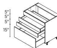
3 DRAWERS / 1 FIXED FRONT 36" | BCT4D36FF
