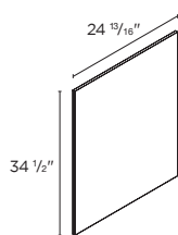
BASE CABINET COVER PANEL
