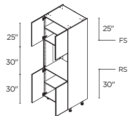
SINGLE OVEN 3 4 DOORS 30" | TO3089.5
