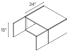
15" HIGH 2 DOORS 30" | W301524 36" | W361524
