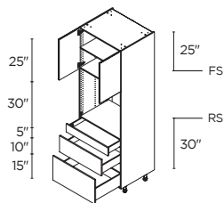
SINGLE OVEN 3 2 DOORS / 3 DRAWERS 30" | TO3D3089.5
