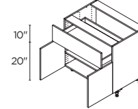
2 DOORS / 1 DRAWER 36" | BCT36A
